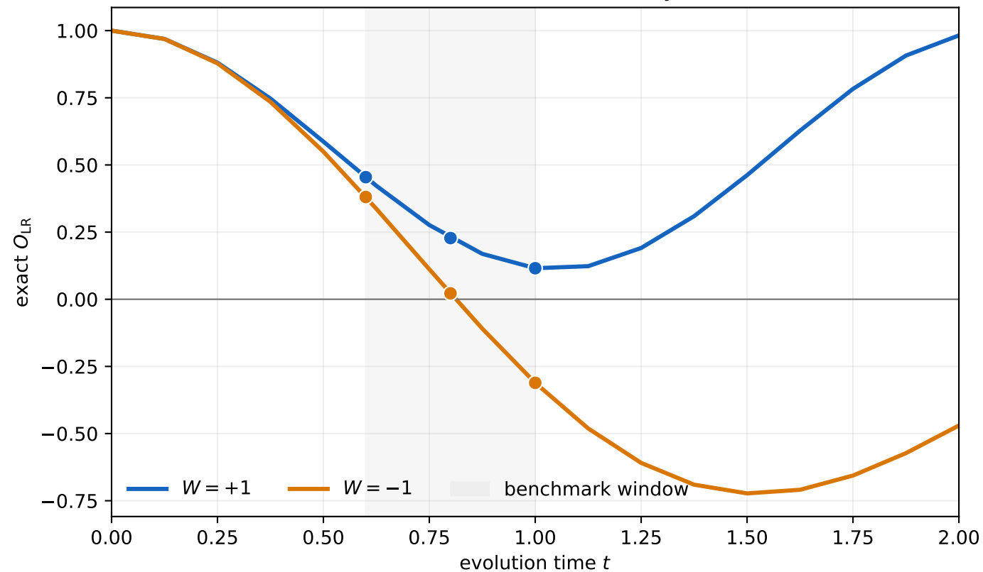
Exact sector-resolved matter dynamics
