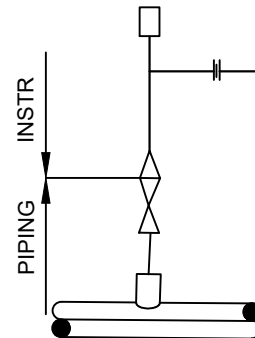
DETAIL - 2 ALTERNATIVE INSTALLATION FOR LIQUID & GAS SERVICES
