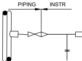
DETAIL - 1 ALTERNATIVE INSTALLATION FOR LIQUID & STEAM SERVICES
