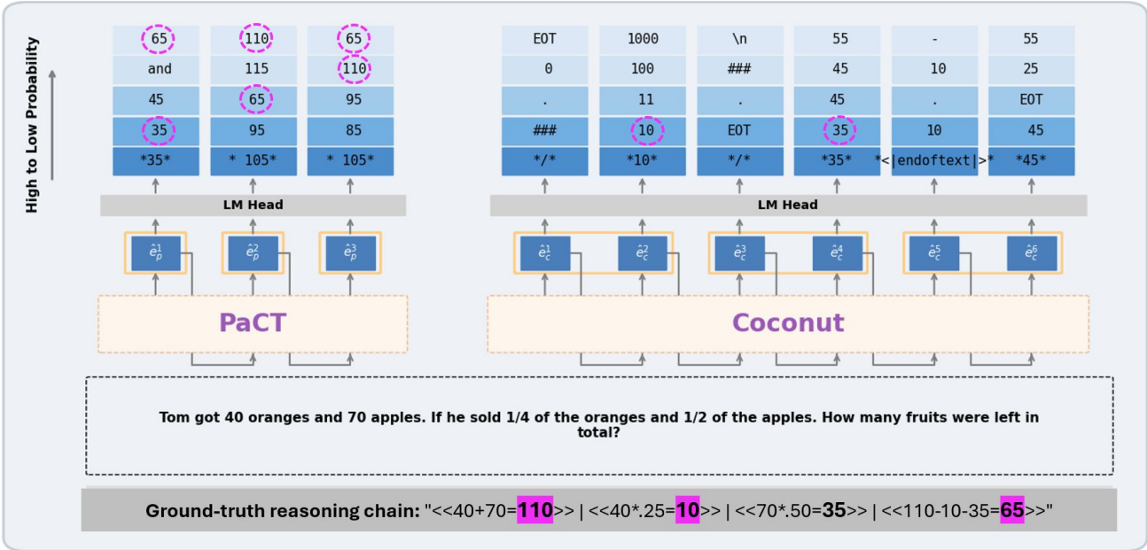
Figure 11. PaCT vs Coconut latent decoding comparison - example 3
