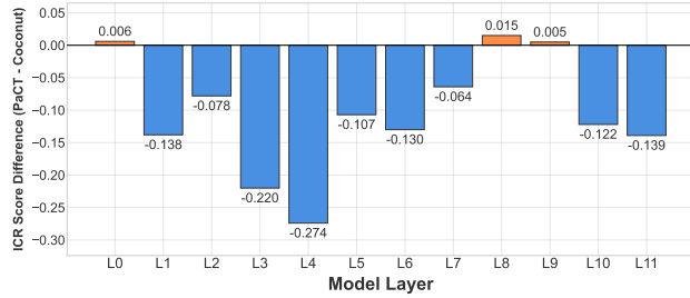
Figure 7. Layer-wise difference in ICR scores between PaCT and CoCoNut. Negative values indicate lower ICR for PaCT.
