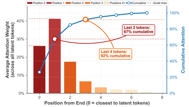
Figure 8. Cross-attention weight distribution across different number of context tokens. Position 0 denotes the last token before latent synthesis, position 1 the second-to-last, and so on. The model concentrates attention on the most recent 1–2 positions regardless of available context.
