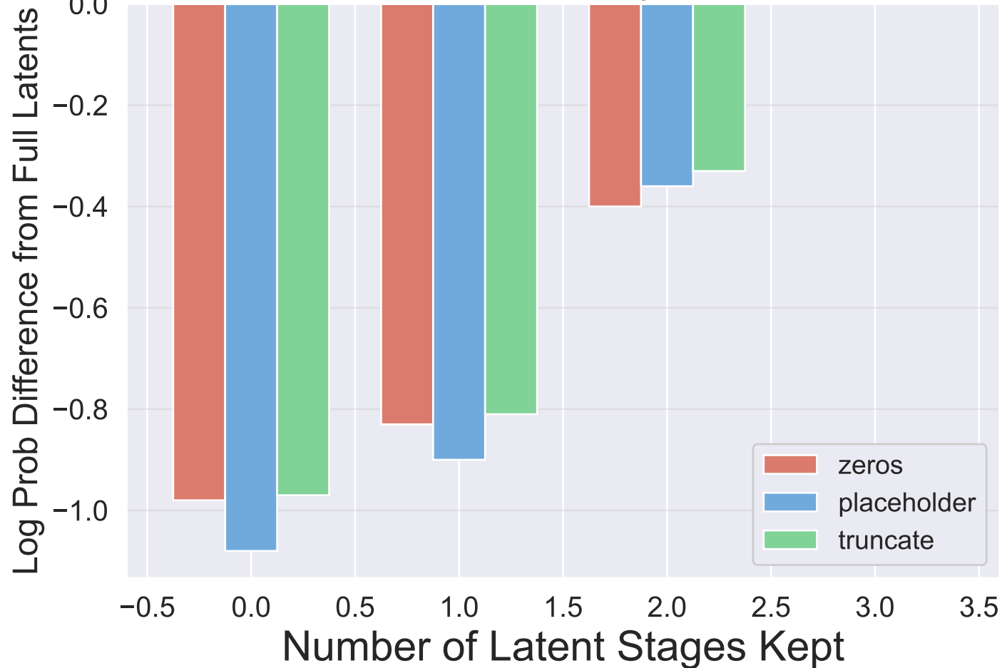
Generated Answer: Probability Loss from Ablation
