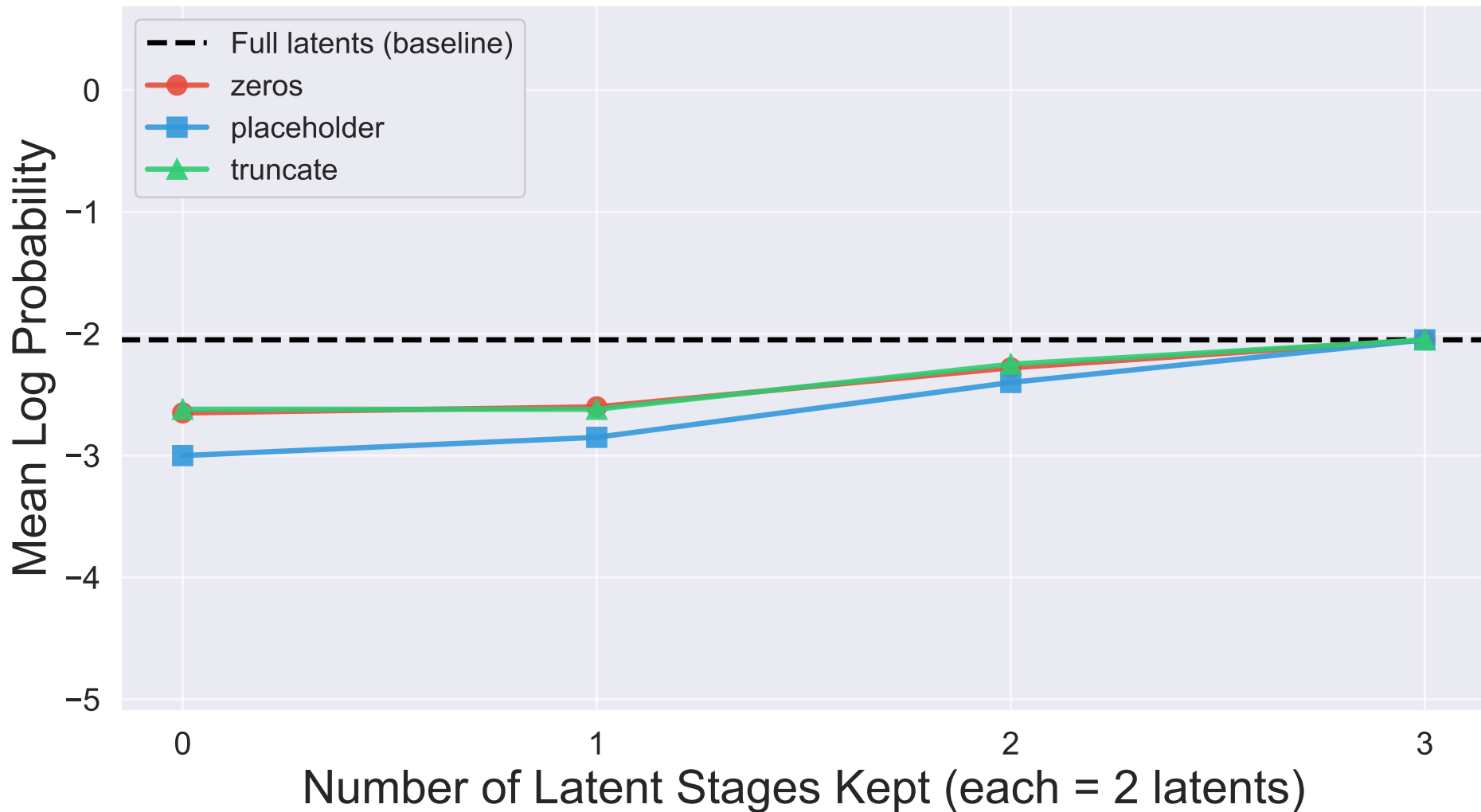
Ground Truth Answer Probability vs Latent Stages
