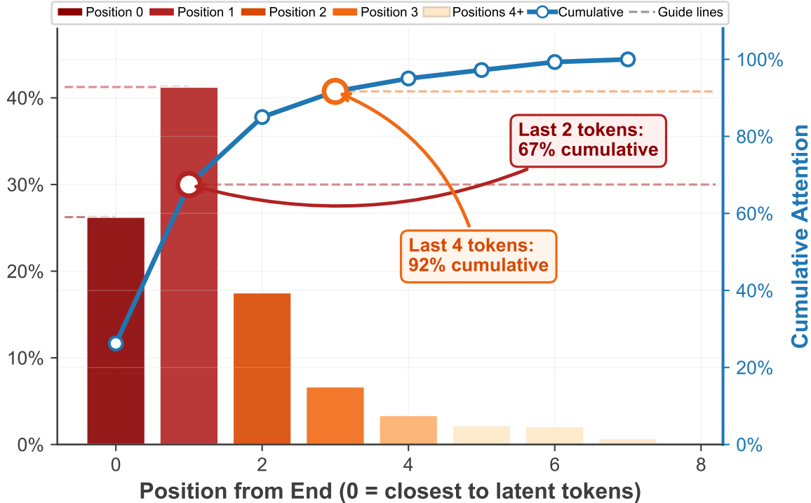
Average Attention Weight (across all latent tokens)
