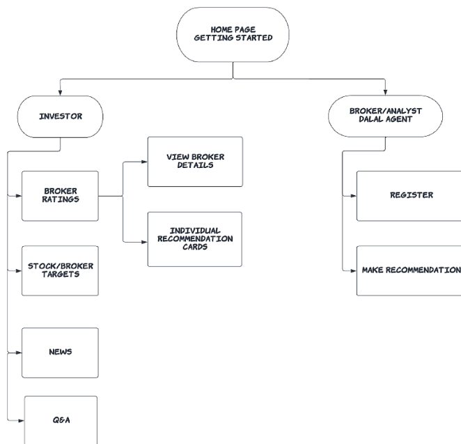
Fig. 3. User Navigation
