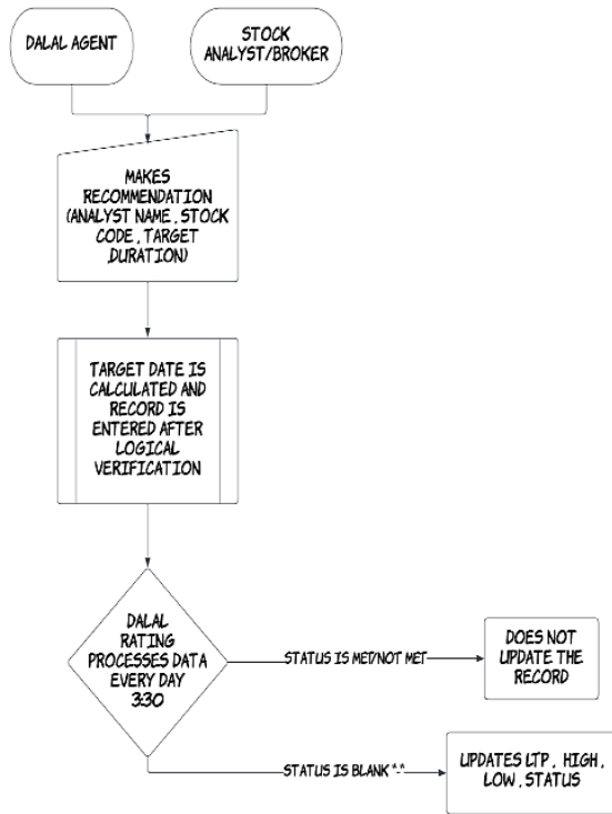
Fig. 2. Proposed Methodology
