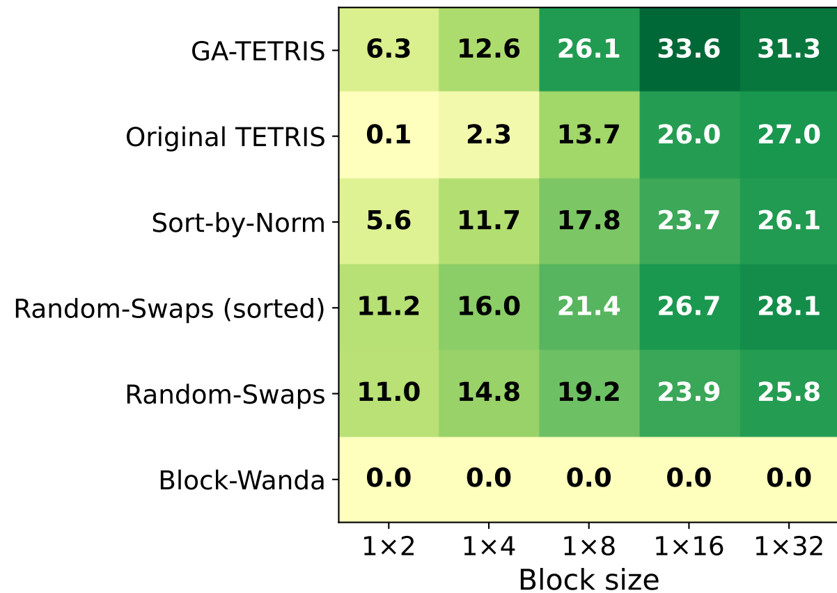
Small ViT
