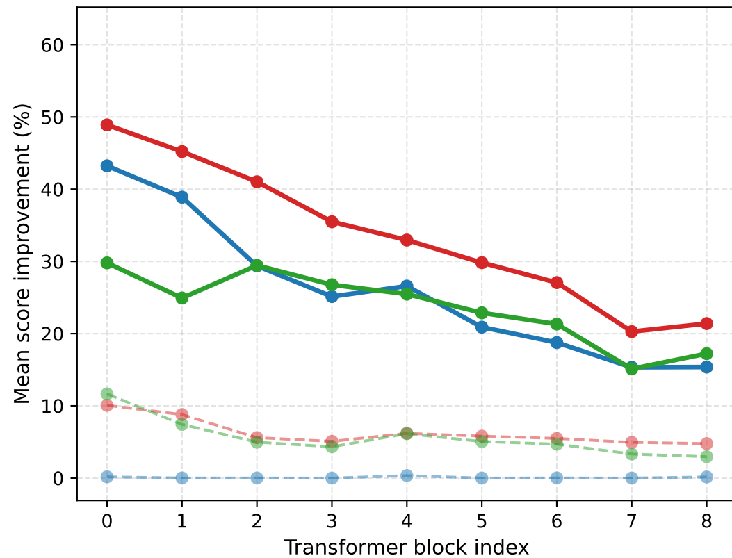
Small ViT
