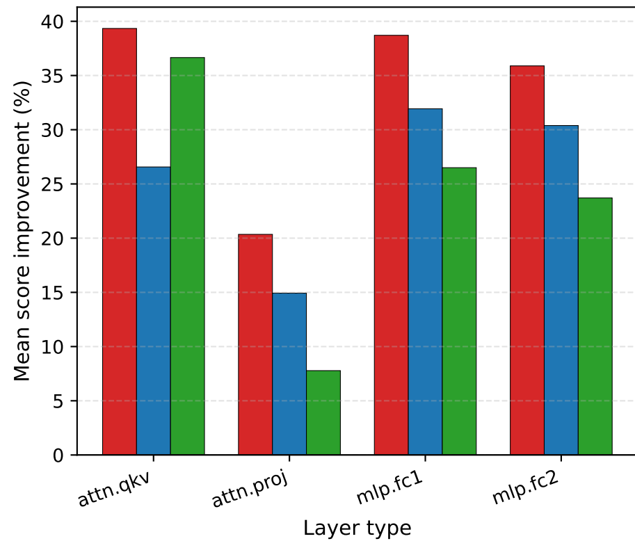
Small ViT
