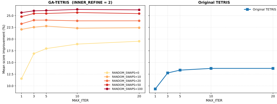
Figure 3.1: Score improvement tradeoff for Original TETRIS and GA-TETRIS as a function of iteration count. With block shape 1 \times 8 on the Small ViT.
