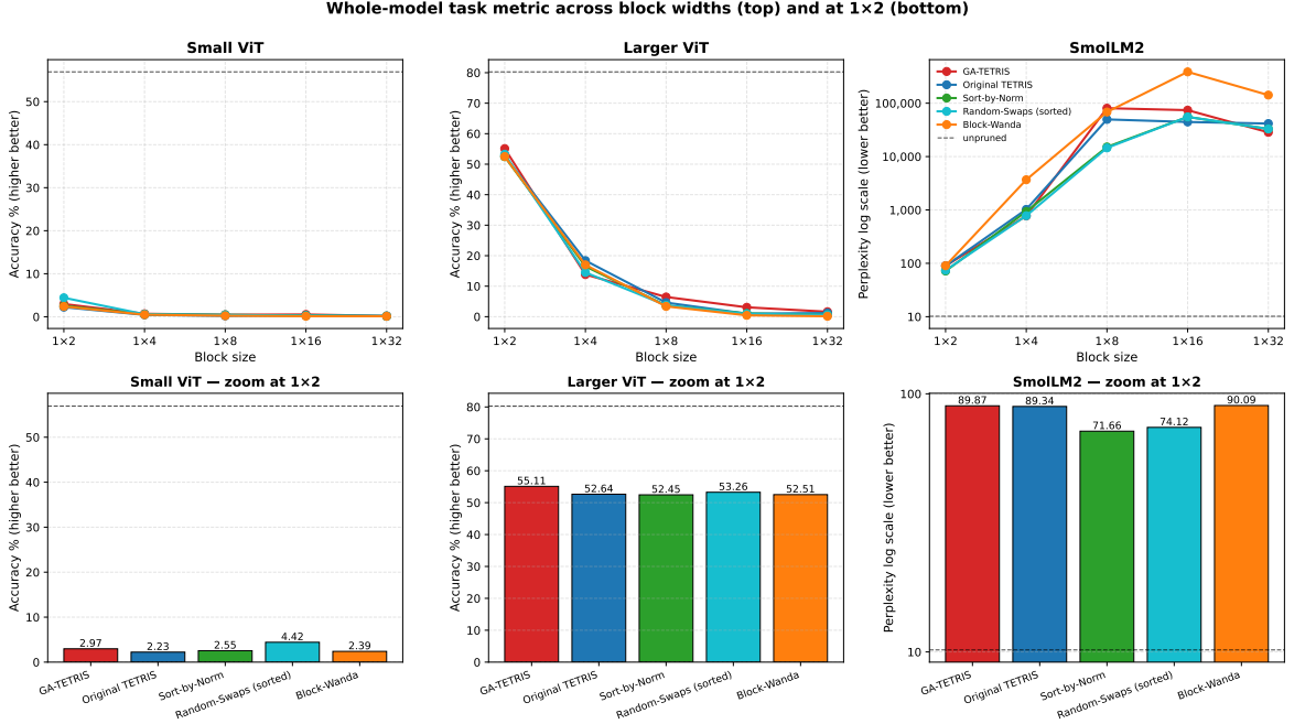
Figure 3.6: Whole-model performance after pruning across block widths and models and zoom on 1 \times 2 block shape.
