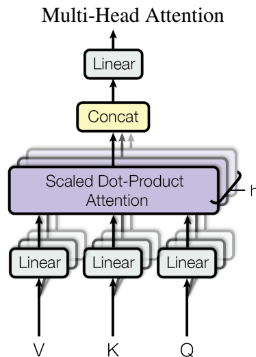
Figure 1.2: Multi-Head Attention mechanism diagram. Adapted from [25].
