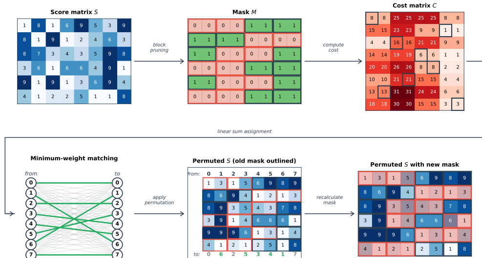
Figure 2.4: One phase-1 iteration of GA-TETRIS (with noise disabled), followed by the beginning of the next iteration
