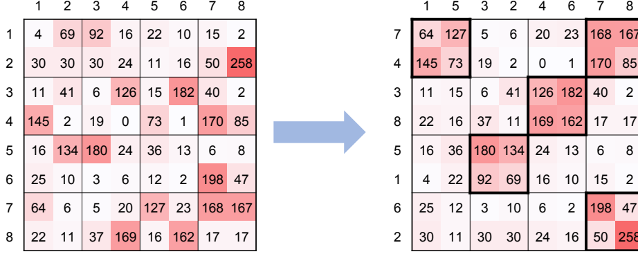
Figure 1.4: The permutations applied by TETRIS to group important elements together. Adapted from [14].
