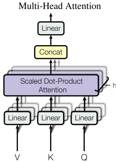
Figure 1.2: Multi-Head Attention mechanism diagram. Adapted from [24].
