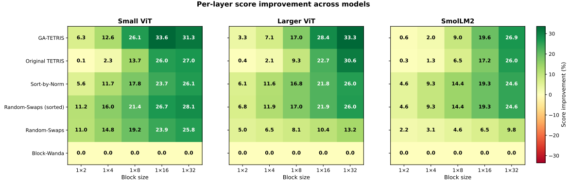
Figure 3.2: Mean (layer-wise) score improvement (%) on all models.
