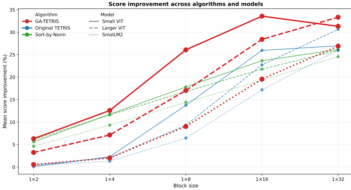
Figure 3.3: Mean (layer-wise) score improvement (%) of selected algorithms across block widths and models.
