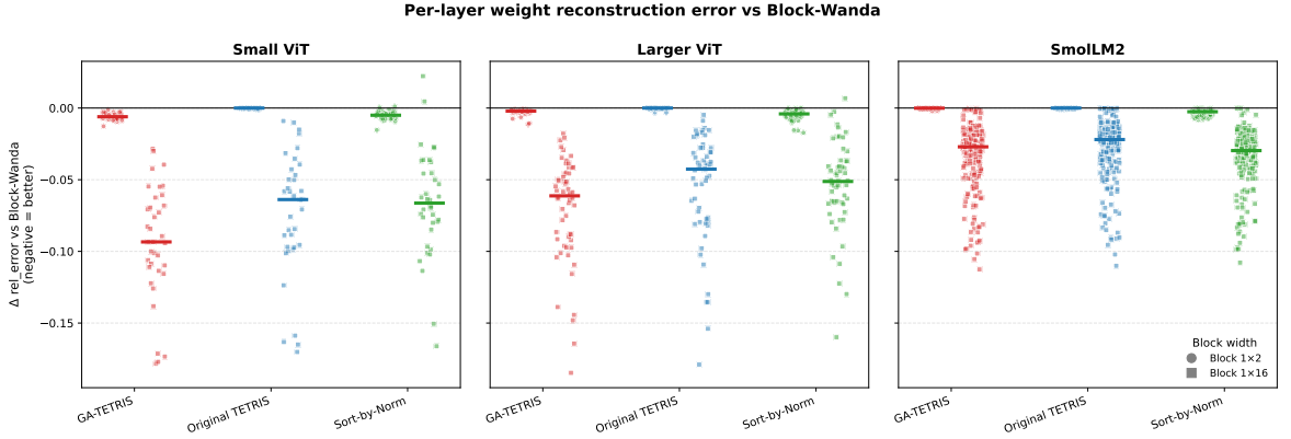
Figure 3.6: Per-layer \Delta\text{rel\_error} of selected algorithms against the Block-Wanda baseline. Each dot is one layer; the horizontal bar marks the median.
