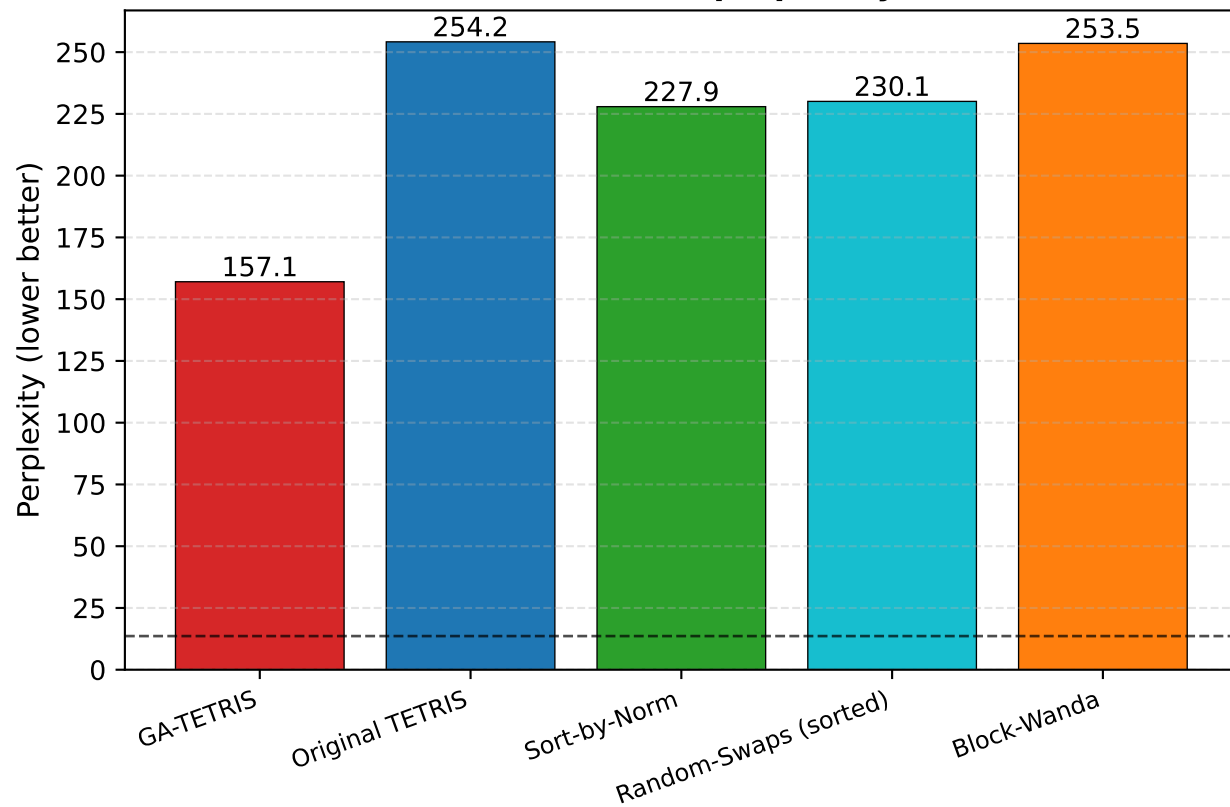
Whole-model perplexity
