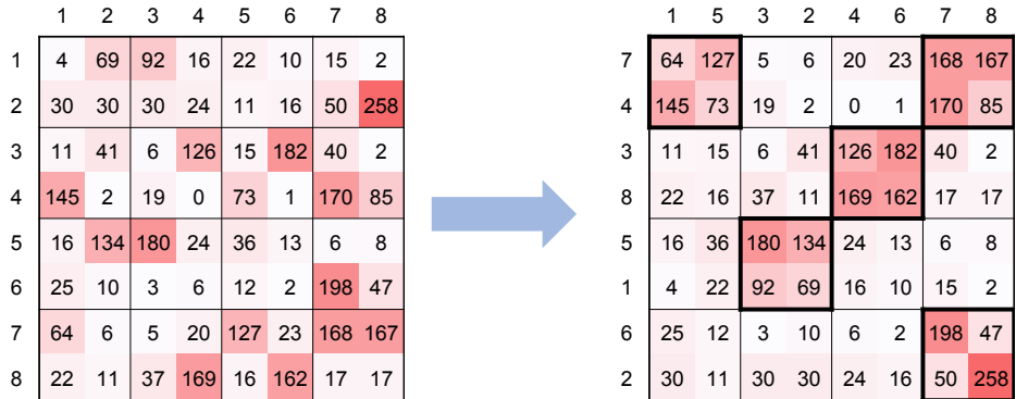
Figure 1.5: The permutations applied by TETRIS to group important elements together. Adapted from [15].
