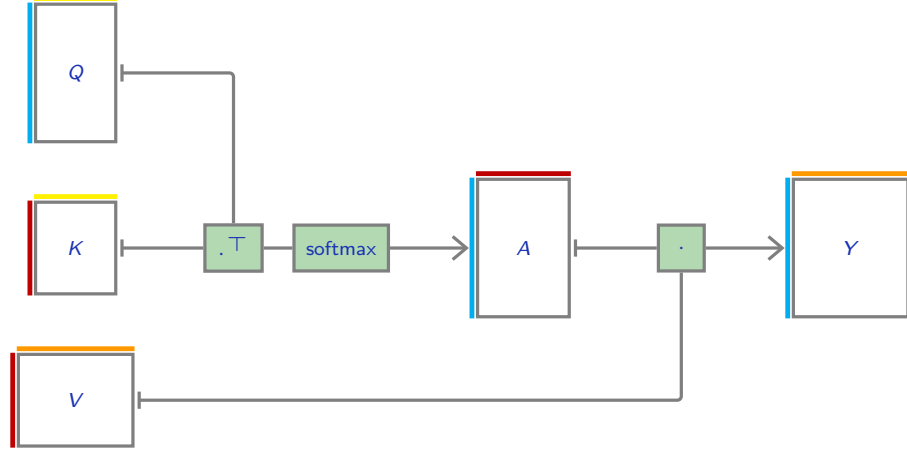
Figure 1.1: Self-attention mechanism diagram. Adapted from Fleuret (2024).
