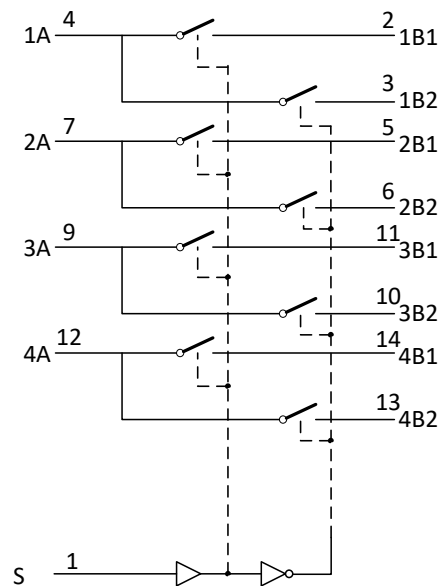
Fig. 1. Logic diagram
