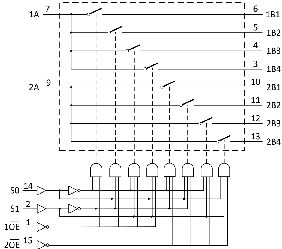
Fig. 1. Logic diagram
