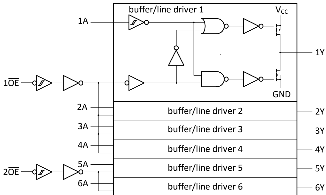
Fig. 3. Logic diagram
