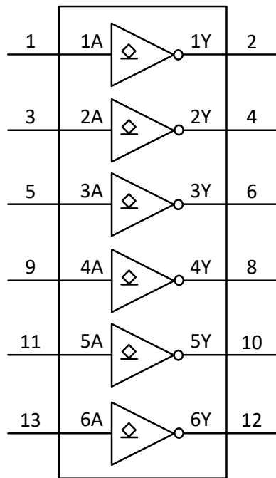
Fig. 1. Logic symbol
