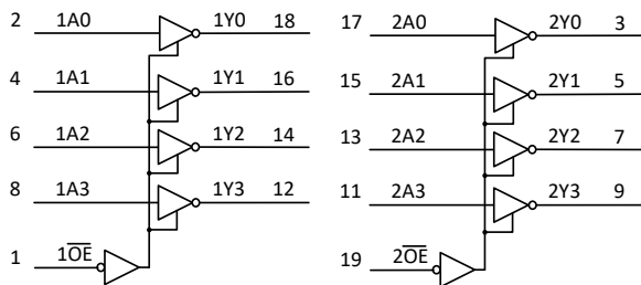
Fig. 2. Logic symbol
