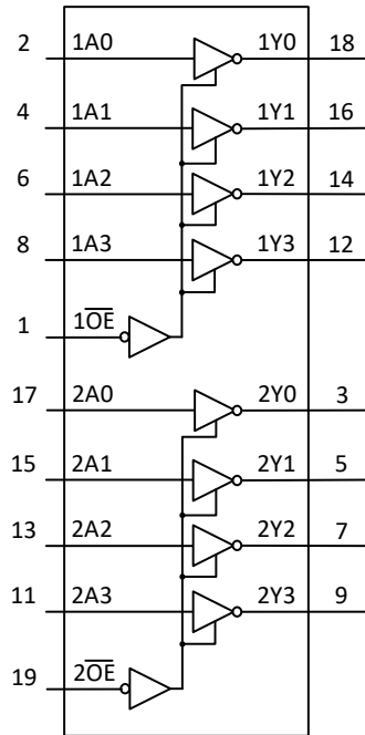
Fig. 1. Functional diagram
