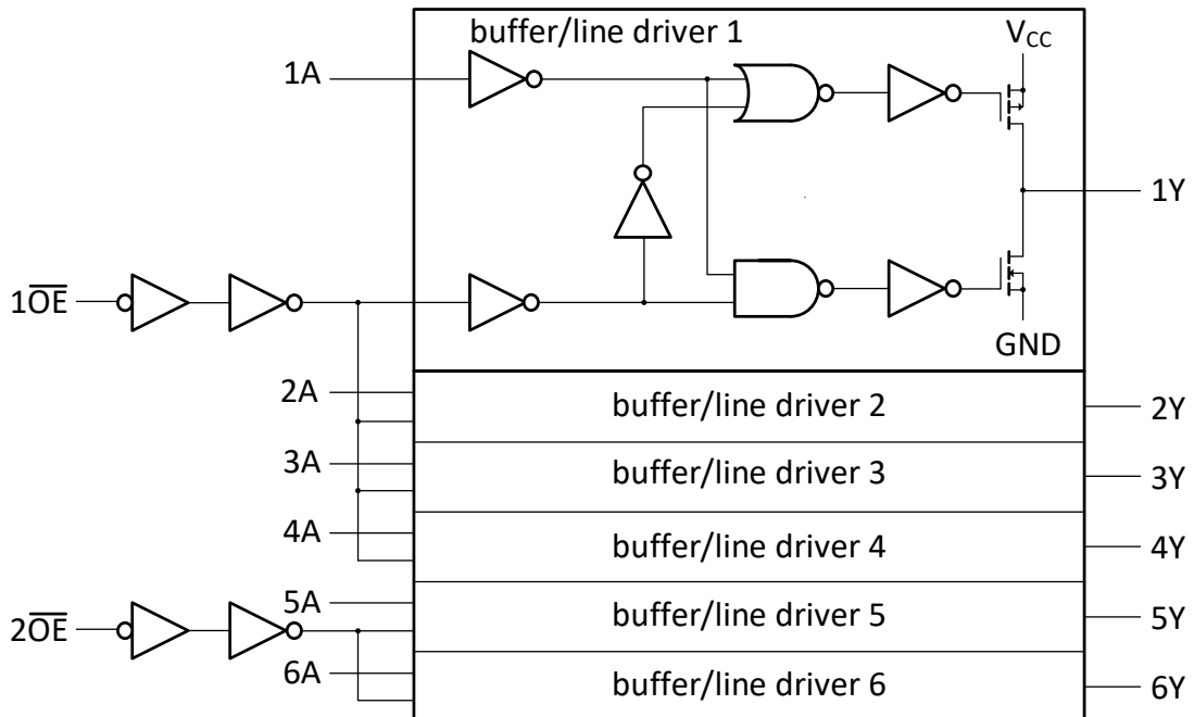
Fig. 3. Logic diagram
