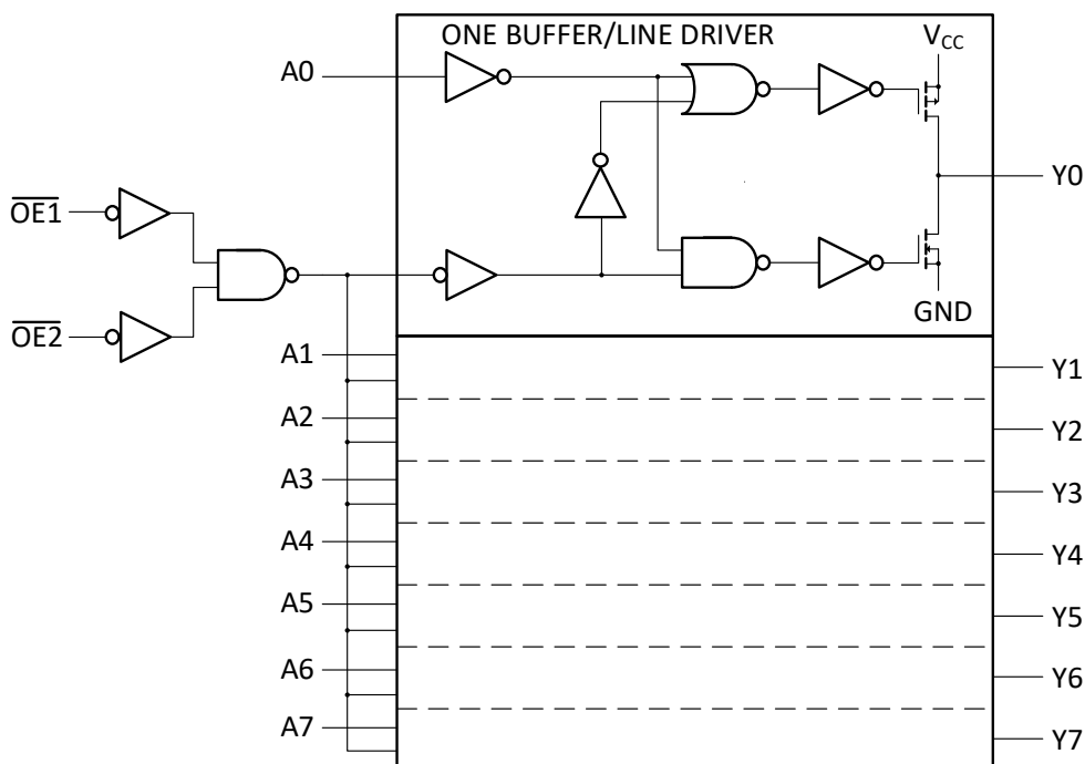
Fig. 4. Logic diagram
