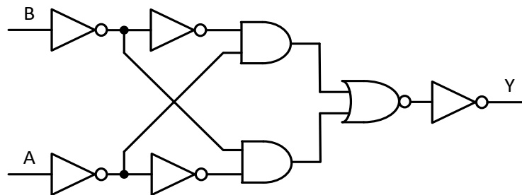
Fig. 3. Logic diagram
