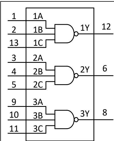
Fig. 1. Logic symbol
