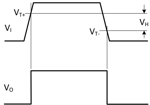
Fig. 15. Definition of V_{T+} , V_{T-} and V_H
