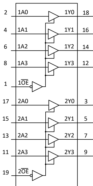
Fig. 1. Functional diagram
