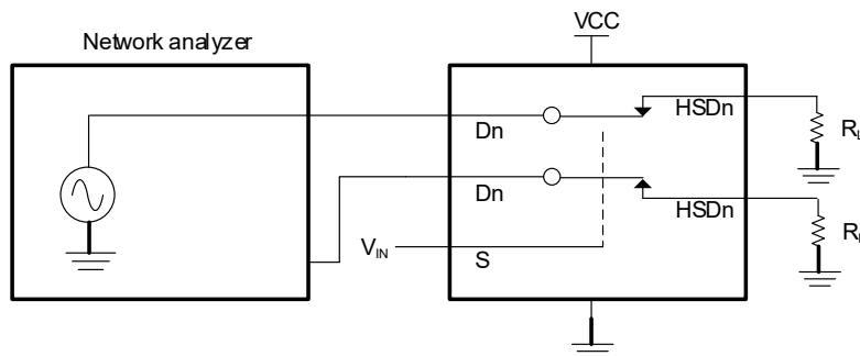
Fig 7. Crosstalk
