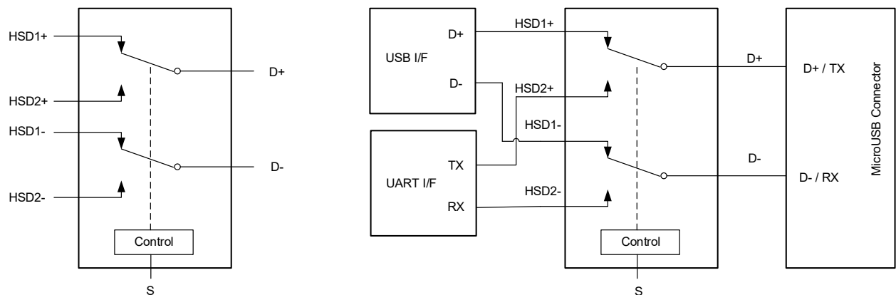
Fig 2. USB2.0 Switch
