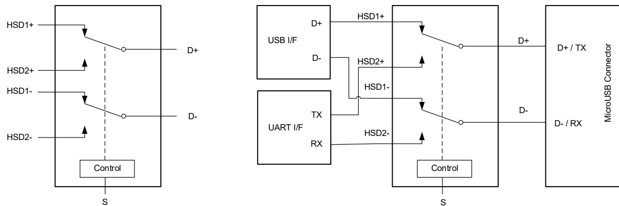
Fig 3. USB2.0 Switch
