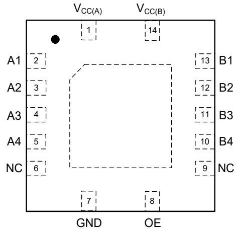
Fig. 3. Top view pin configuration QFN14L
