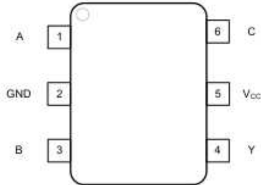
Fig. 4. Top view pin configuration SOT23-6L, SOT363
