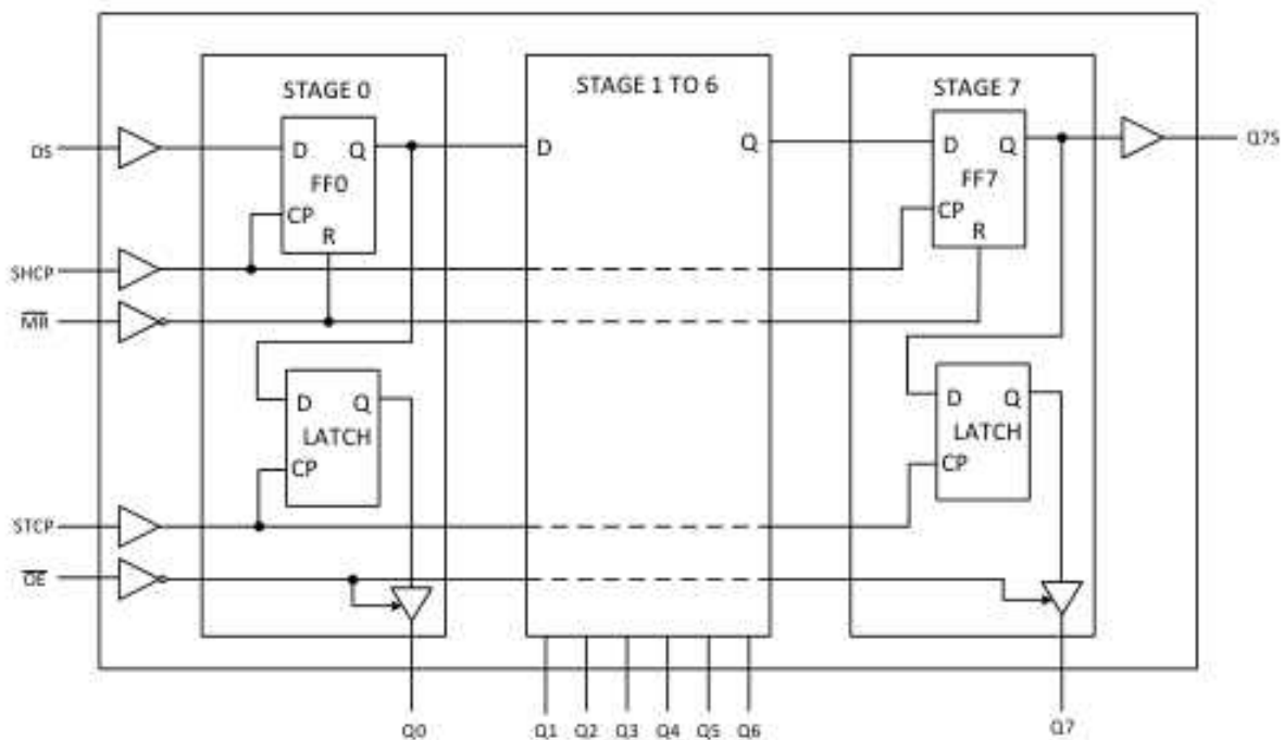
Fig. 4. Logic diagram
