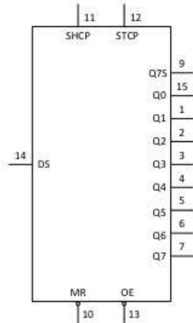
Fig. 2. Logic symbol
