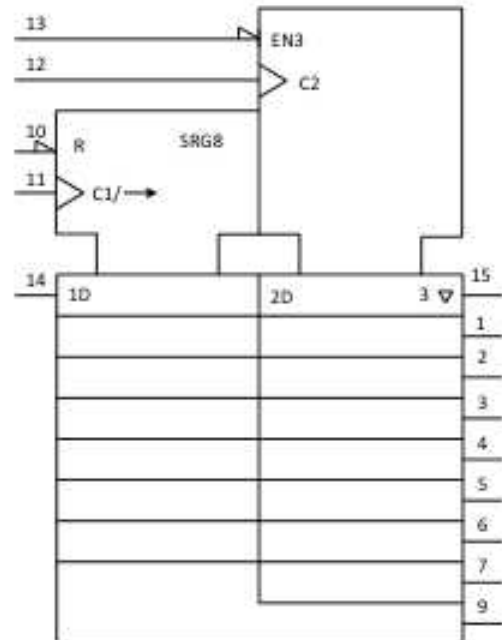
Fig. 3. IEC logic symbol
