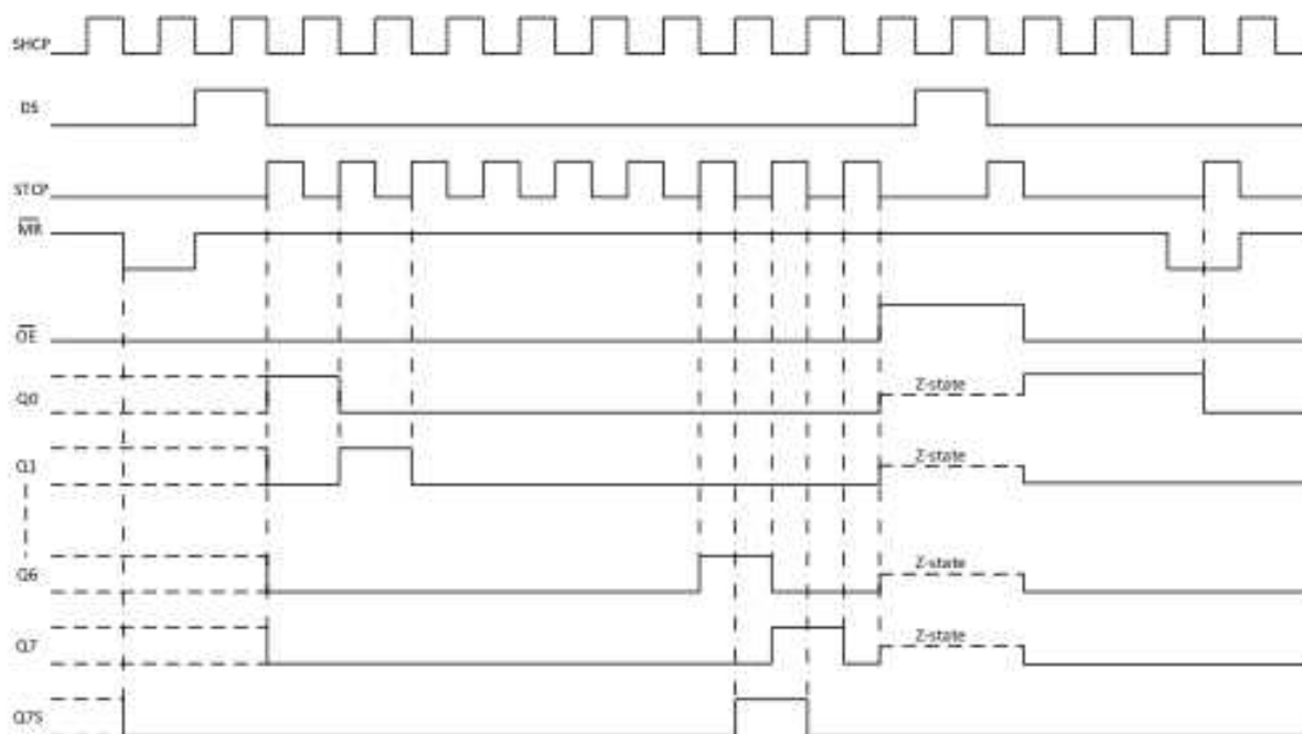
Fig. 6. Timing diagram
