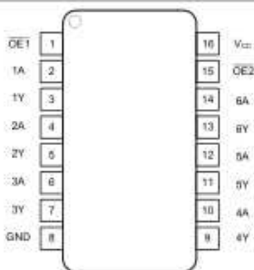
Fig. 5. Top view pin configuration SOP and TSSOP
