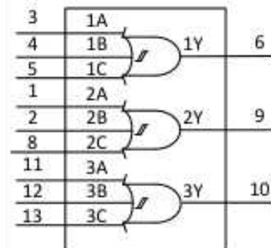
Fig. 1. Logic symbol
