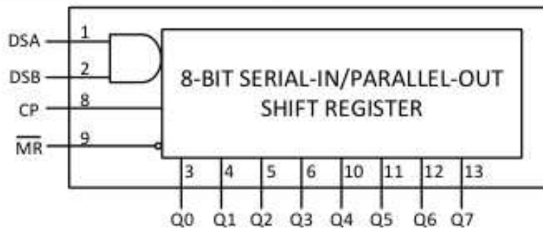
Fig. 3. Logic diagram
