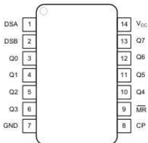
Fig. 5. Top view pin configuration SOP and TSSOP
