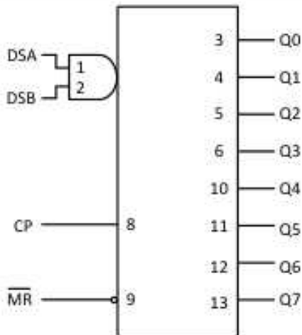
Fig. 1. Logic symbol
