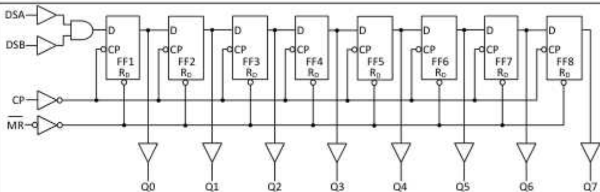
Fig. 4. Functional diagram
