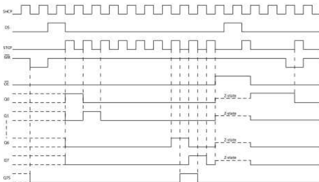
Fig. 6. Timing diagram
