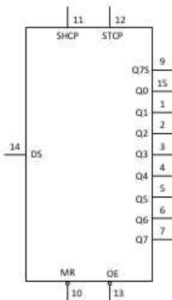
Fig. 2. Logic symbol
