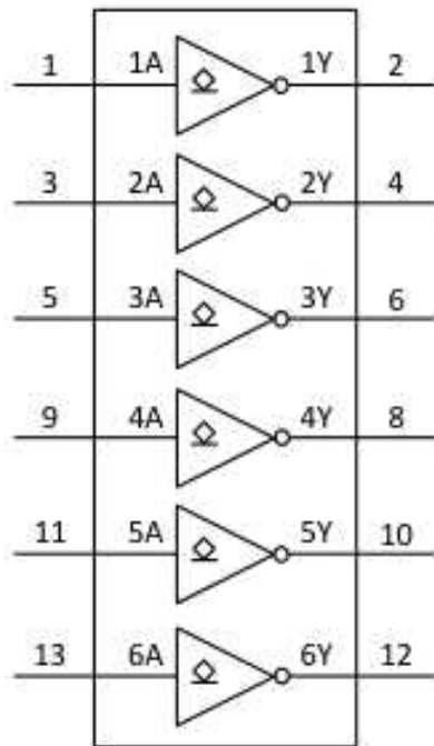
Fig. 1. Logic symbol
