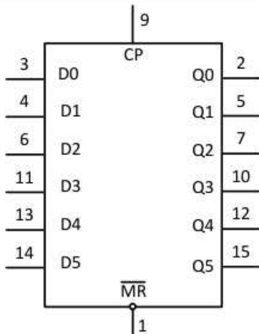
Fig. 1. Logic symbol
