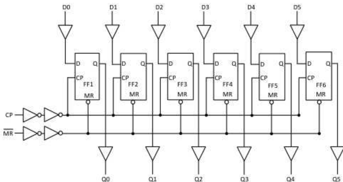
Fig. 3. Logic diagram
