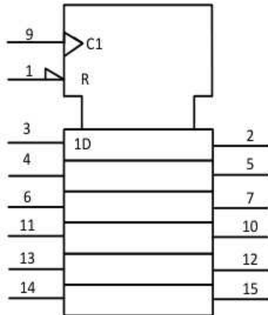
Fig. 2. IEC Logic symbol
