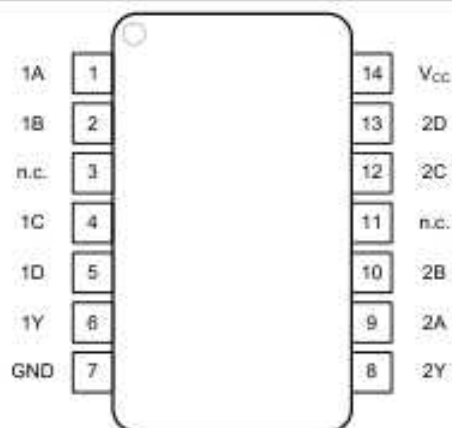
Fig. 4. Top view pin configuration SOP and TSSOP
