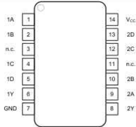
Fig. 4. Top view pin configuration SOP and TSSOP
