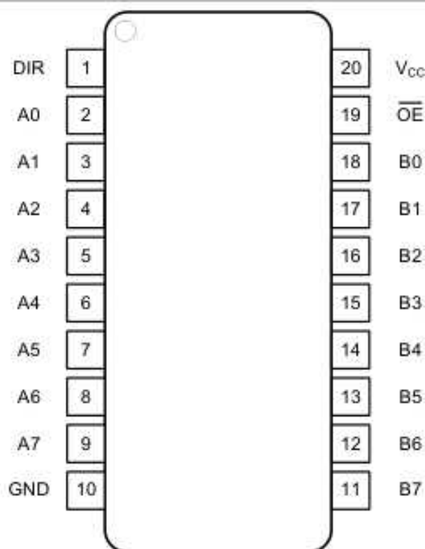
Fig. 3. Top view pin configuration SOP and TSSOP
