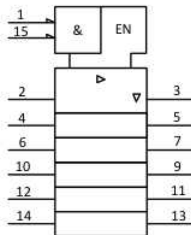
Fig. 3. IEC logic symbol
