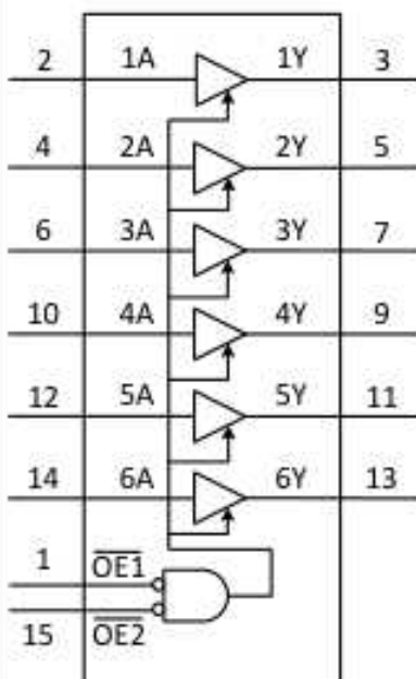
Fig. 1. Functional diagram
