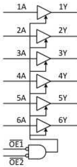
Fig. 2. Logic symbol
