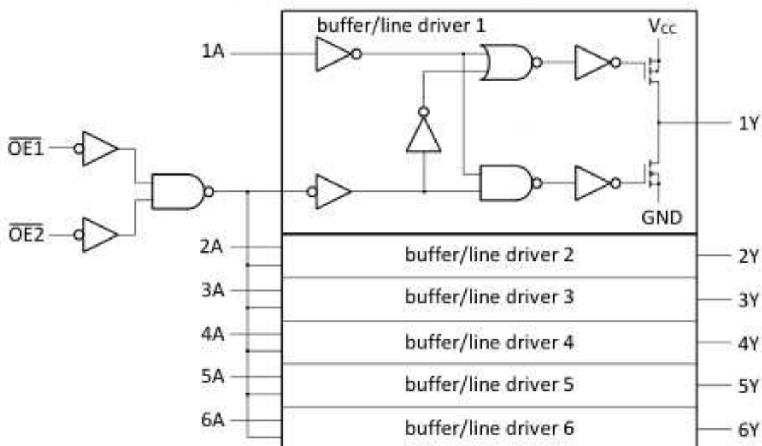
Fig. 4. Logic diagram
