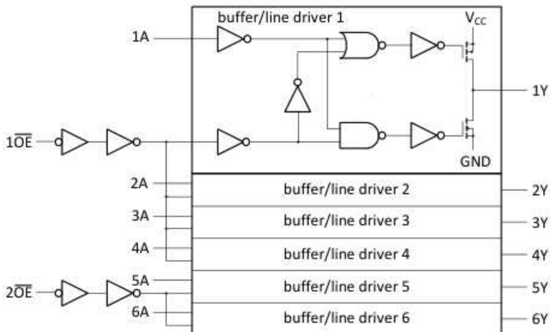
Fig. 3. Logic diagram
