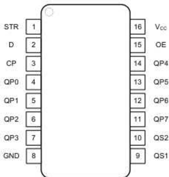
Fig. 5. Top view pin configuration SOP and TSSOP
