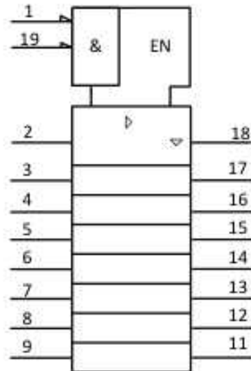
Fig. 2. IEC logic symbol
