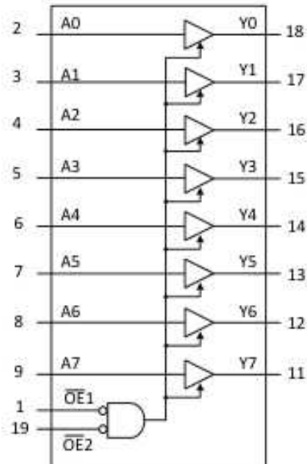
Fig. 3. Functional diagram
