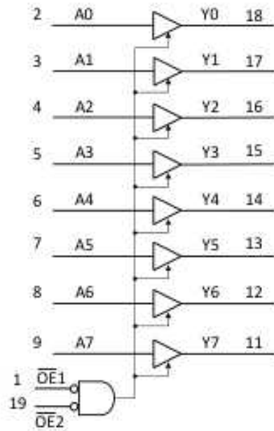
Fig. 1. Logic symbol
