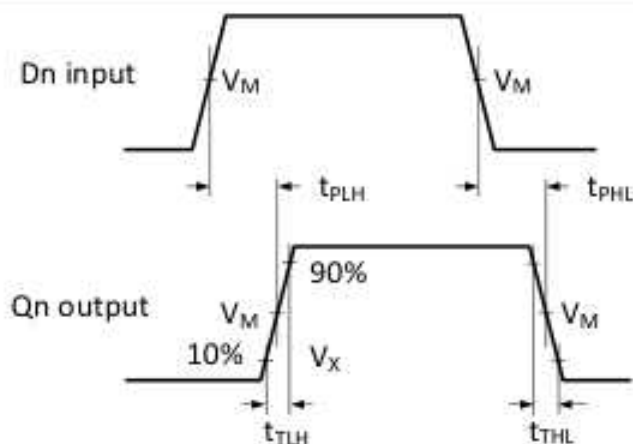
Fig. 6. Propagation delay data input (Dn) to output (Qn) and output transition time
