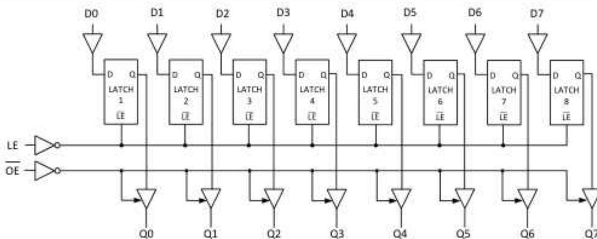
Fig. 2. Functional diagram
