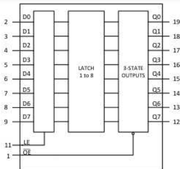
Fig. 1. Logic diagram
