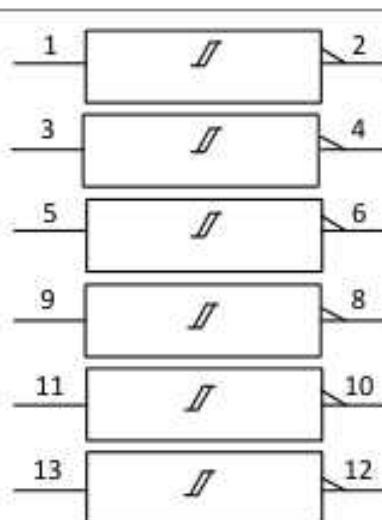
Fig. 2. IEC logic symbol
