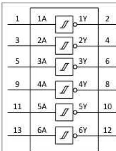
Fig. 1. Logic symbol
