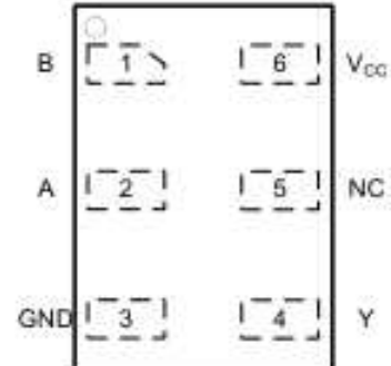
Fig 5. Top view pin configuration DFN6L
