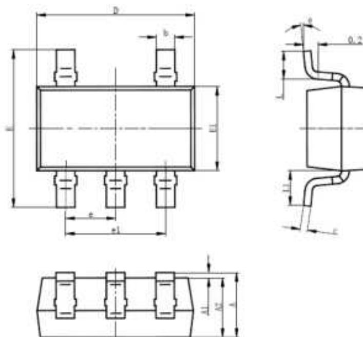
SOT-23-5L(14RZ) PACKAGE OUTLINE DIMENSIONS
