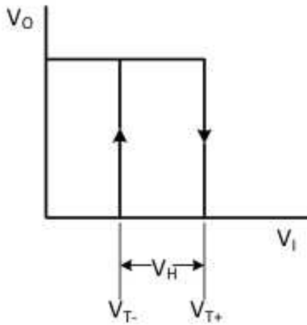
Fig 9. Transfer characteristic
