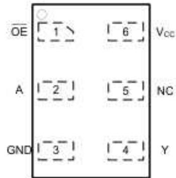
Fig 5. Top view pin configuration DFN6L
